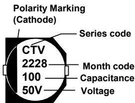
Chip Type Fig.1 ΦD=8~ 10mm
