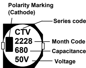
Fig.2 ΦD≥12.5mm
