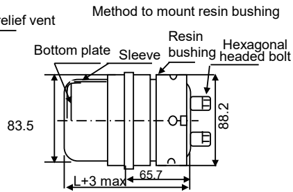
Method to mount resin bushing(ø76)
