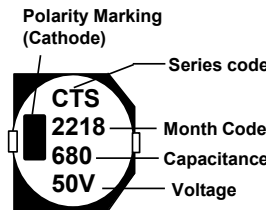
Fig.2 ΦD≥12.5mm
